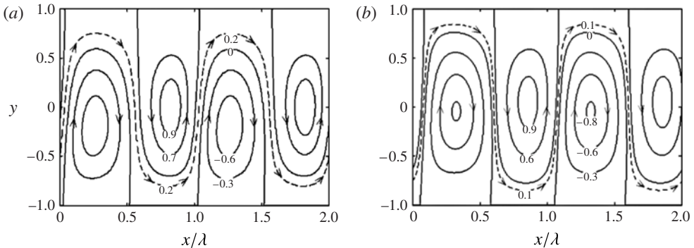
FIGURE 9. Flow topologies for Re = 1 , \alpha = 2 , Ra_{per} = 800 and Ra_{uni}/Ra_{per} = 0 (a, \Psi_{max} = 3.6603 ) and 0.5 (b, \Psi_{max} = 6.8814 ). The corresponding flow conditions correspond to points A and B in figure 8(a).
